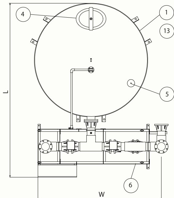
■外形寸法 [Outside dimension]
